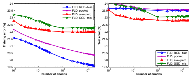
Fig. 4. Training and test errors of stochastic algorithms on pima
