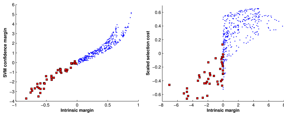
Fig. 1. Correlation between the measures and the intrinsic margin for the NNet dataset with the SVM confidence margin ( Left ) and the Sin dataset with the selection cost ( Right ). Noisy examples with negative intrinsic margins are shown as filled squares.
